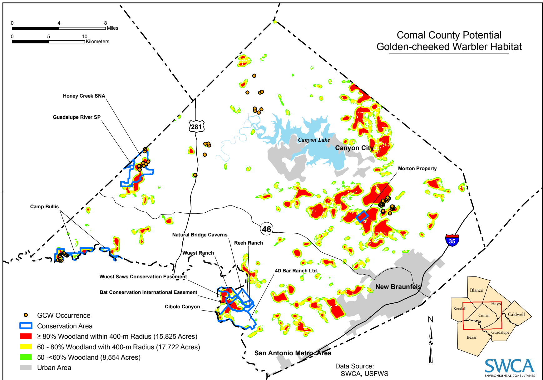
Figure 2-3b. Golden-cheeked warbler (GCW) occurrences, existing conservation areas, and the distribution of potential habitat at 50-<60%, 60-<80%, and ≥ 80% woodlands composition within a 400-meter radius in Comal County, Texas.
